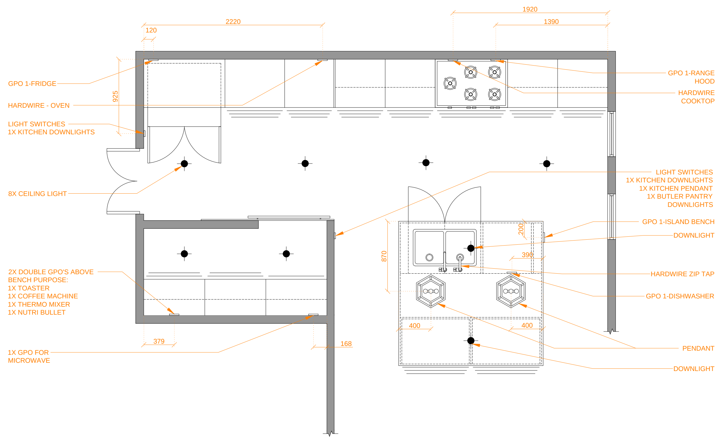
CEILING AND ELECTRICAL PLAN
